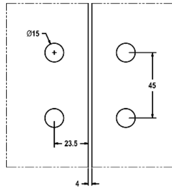
Glass Preparation
